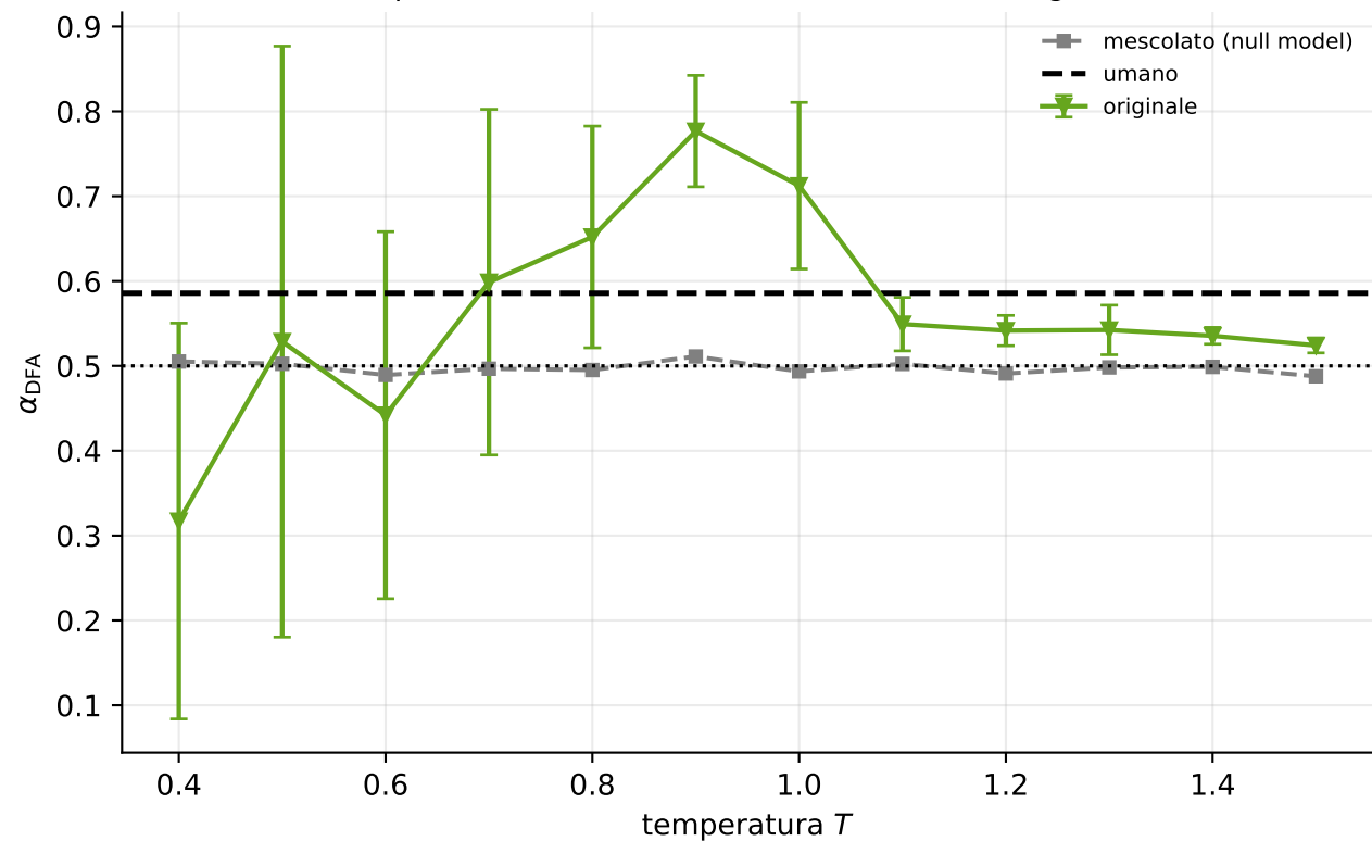
Esponente DFA — Qwen3.5-4B-Base (cfr. [L] Fig. 4B)
